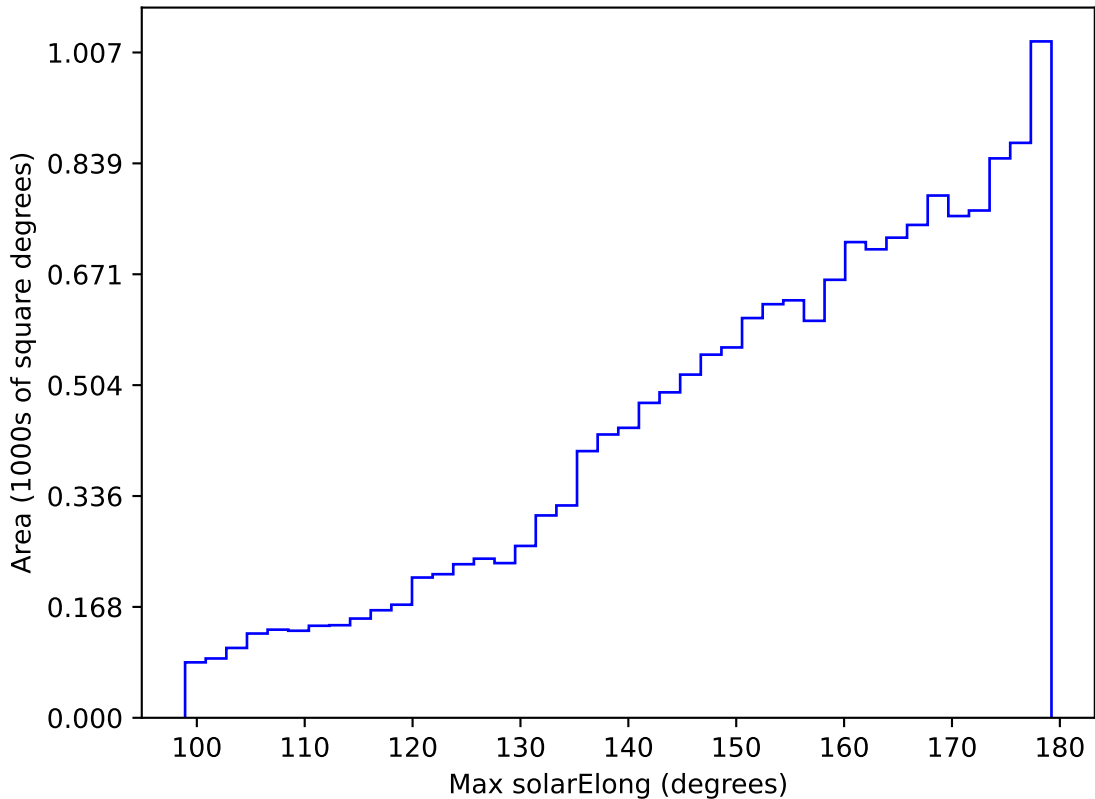
ddf_acor_sf25_lsf30_lsr10_v3.4_10yrs WFD y band: Max solarElong
