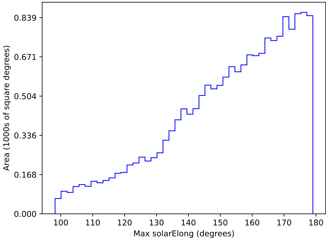
ddf_acor_sf25_lsf30_lsr10_v3.4_10yrs WFD g band: Max solarElong
