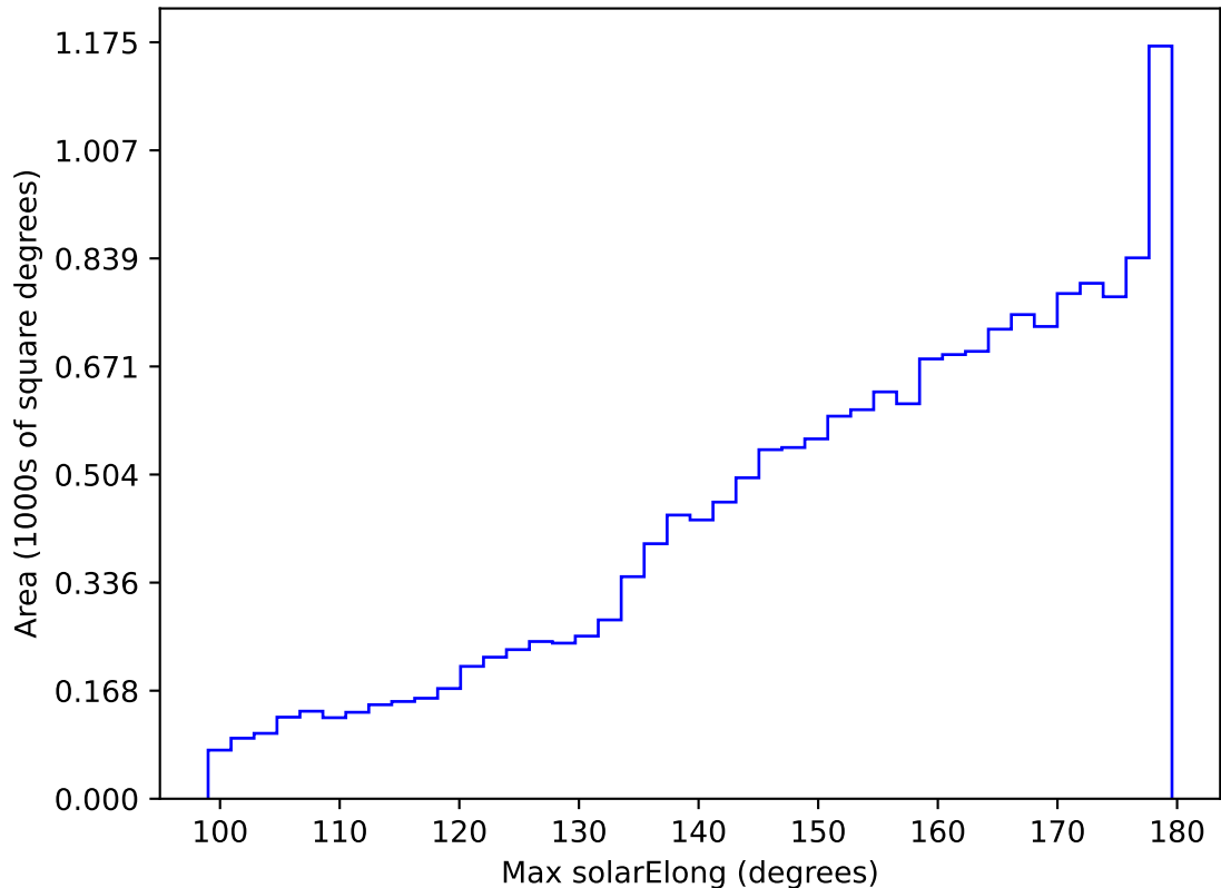
ddf_acor_sf25_lsf30_lsr10_v3.4_10yrs WFD all bands: Max solarElong
