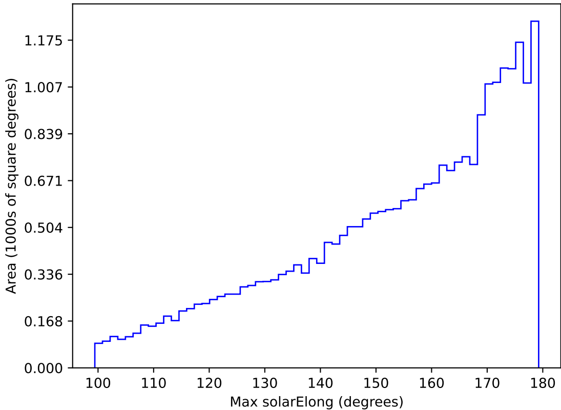
ddf_acor_sf25_lsf30_lsr10_v3.4_10yrs All sky z band: Max solarElong
