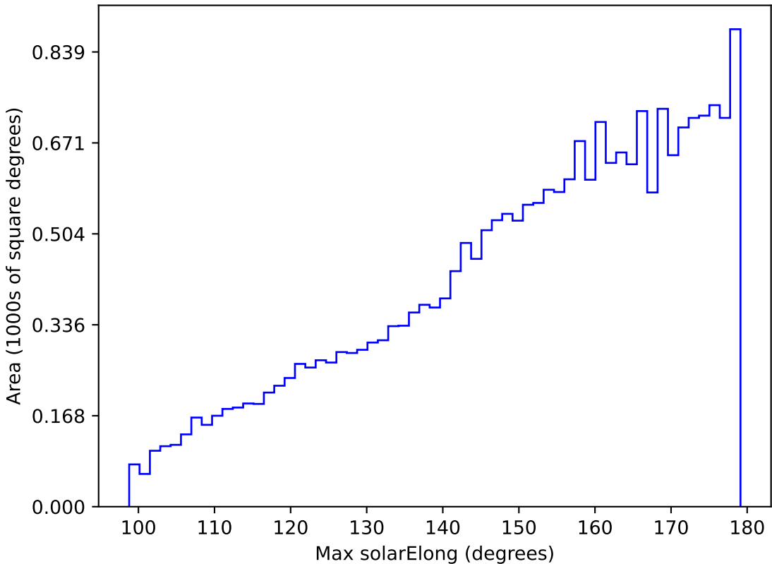
ddf_acor_sf25_lsf30_lsr10_v3.4_10yrs All sky y band: Max solarElong
