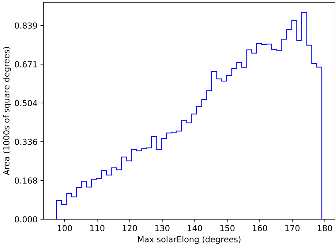
ddf_acor_sf25_lsf30_lsr10_v3.4_10yrs All sky u band: Max solarElong
