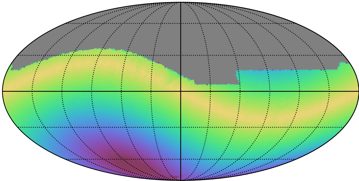
ddf_acor_sf25_lsf30_lsr10_v3.4_10yrs All sky r band: Max solarElong
