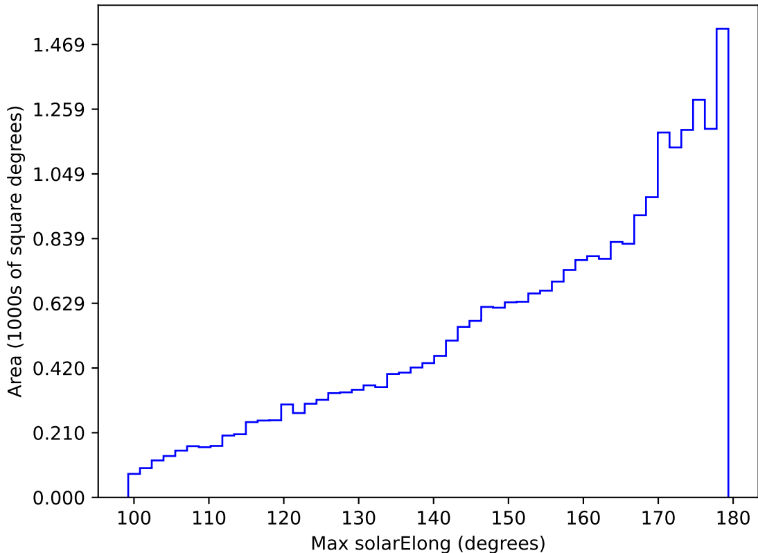
ddf_acor_sf25_lsf30_lsr10_v3.4_10yrs All sky r band: Max solarElong
