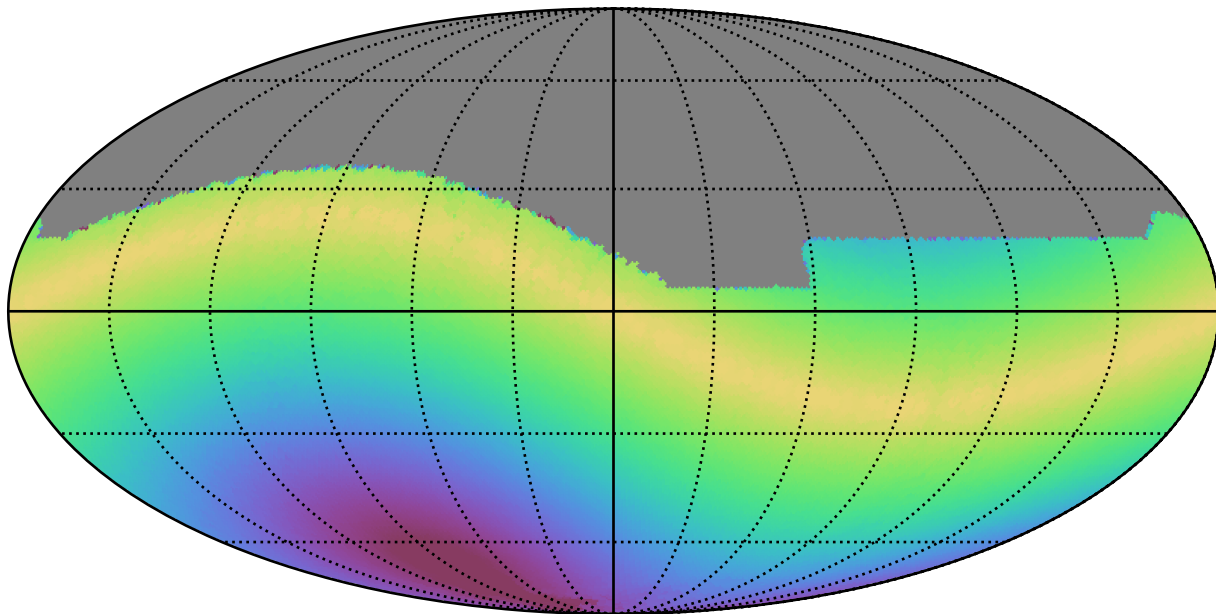
ddf_acor_sf25_lsf30_lsr10_v3.4_10yrs All sky i band: Max solarElong
