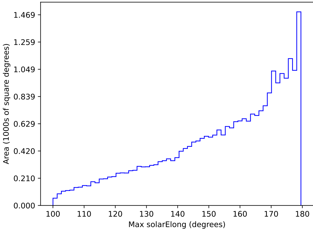
ddf_acor_sf25_lsf30_lsr10_v3.4_10yrs All sky all bands: Max solarElong
