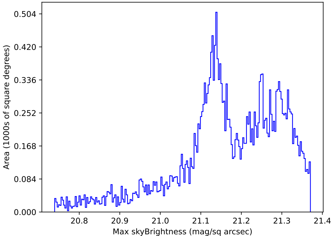
ddf_acor_sf25_lsf30_lsr10_v3.4_10yrs Yr 1 r band: Max skyBrightness
