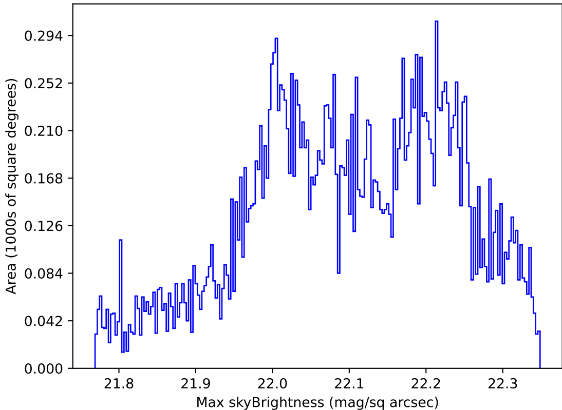
ddf_acor_sf25_lsf30_lsr10_v3.4_10yrs Yr 1 g band: Max skyBrightness
