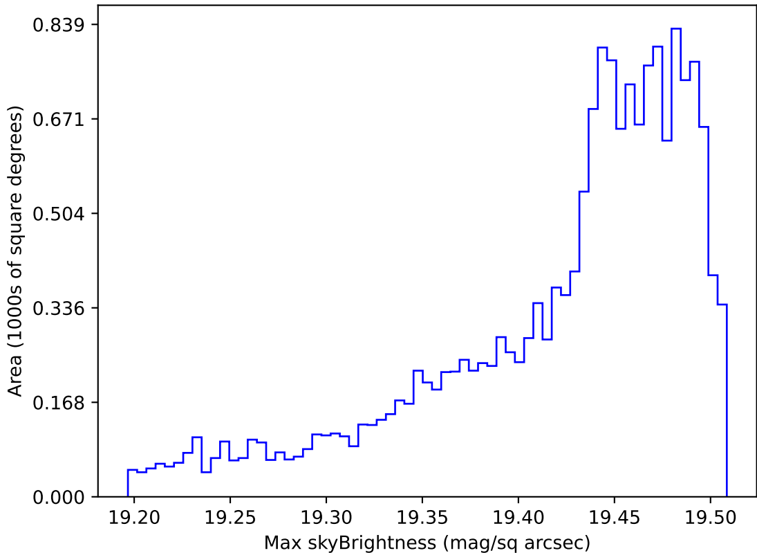
ddf_acor_sf25_lsf30_lsr10_v3.4_10yrs WFD z band: Max skyBrightness
