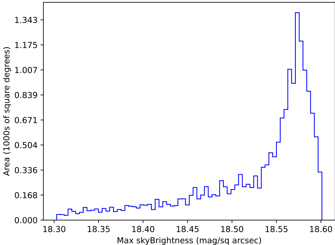
ddf_acor_sf25_lsf30_lsr10_v3.4_10yrs WFD y band: Max skyBrightness
