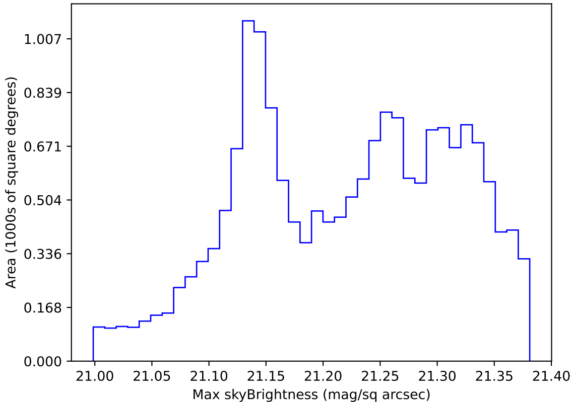
ddf_acor_sf25_lsf30_lsr10_v3.4_10yrs WFD r band: Max skyBrightness
