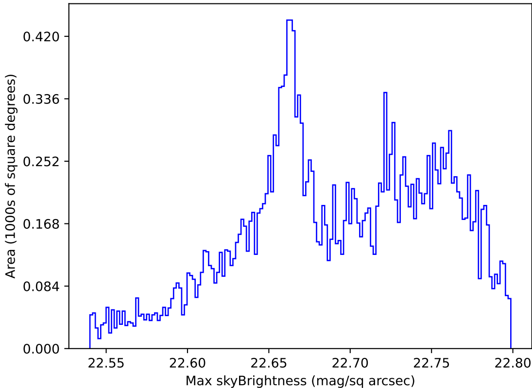
ddf_acor_sf25_lsf30_lsr10_v3.4_10yrs All sky u band: Max skyBrightness
