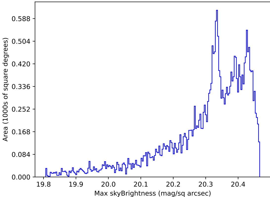
ddf_acor_sf25_lsf30_lsr10_v3.4_10yrs All sky i band: Max skyBrightness
