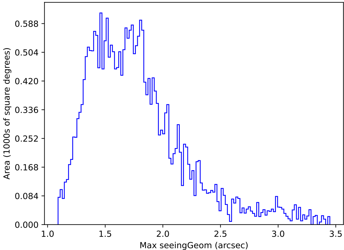
ddf_acor_sf25_lsf30_lsr10_v3.4_10yrs Yr 1 all bands: Max seeingGeom
