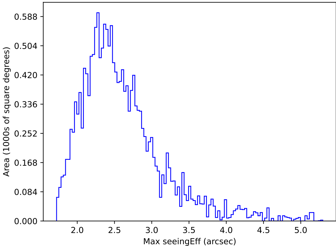
ddf_acor_sf25_lsf30_lsr10_v3.4_10yrs WFD z band: Max seeingEff
