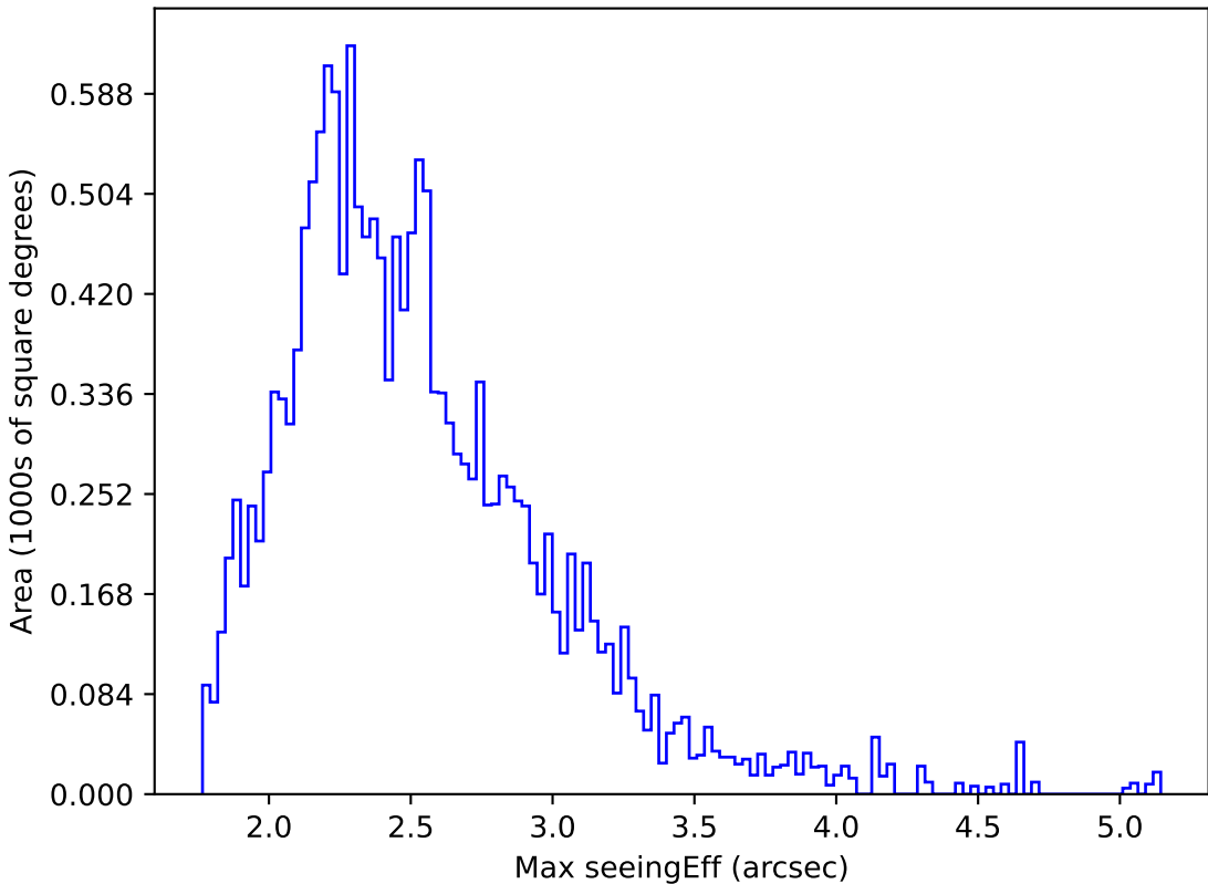
ddf_acor_sf25_lsf30_lsr10_v3.4_10yrs WFD u band: Max seeingEff
