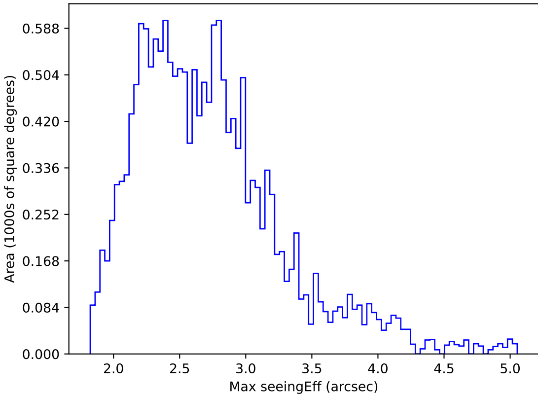
ddf_acor_sf25_lsf30_lsr10_v3.4_10yrs WFD r band: Max seeingEff
