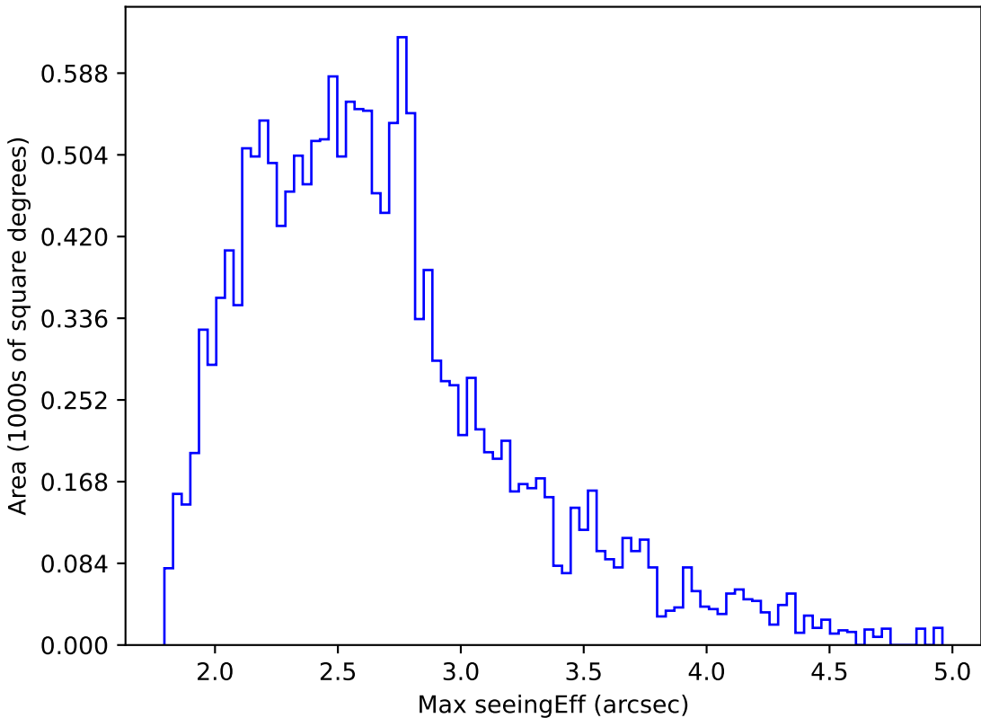
ddf_acor_sf25_lsf30_lsr10_v3.4_10yrs WFD i band: Max seeingEff
