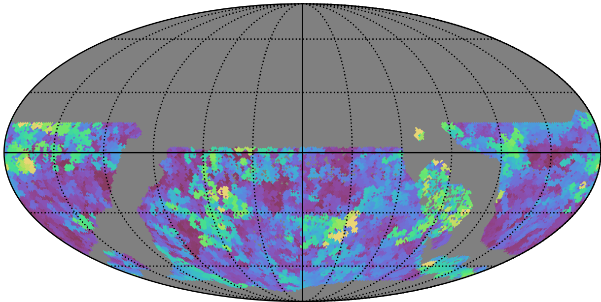
ddf_acor_sf25_lsf30_lsr10_v3.4_10yrs WFD g band: Max seeingEff
