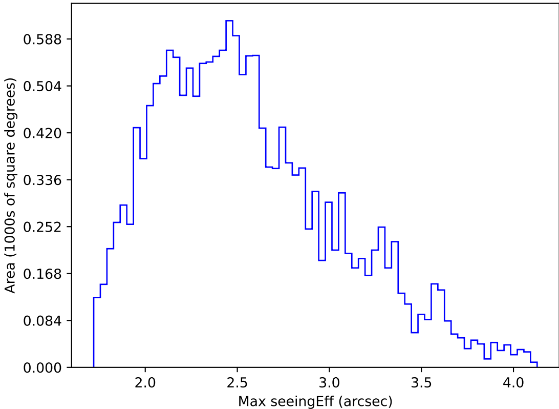
ddf_acor_sf25_lsf30_lsr10_v3.4_10yrs WFD g band: Max seeingEff
