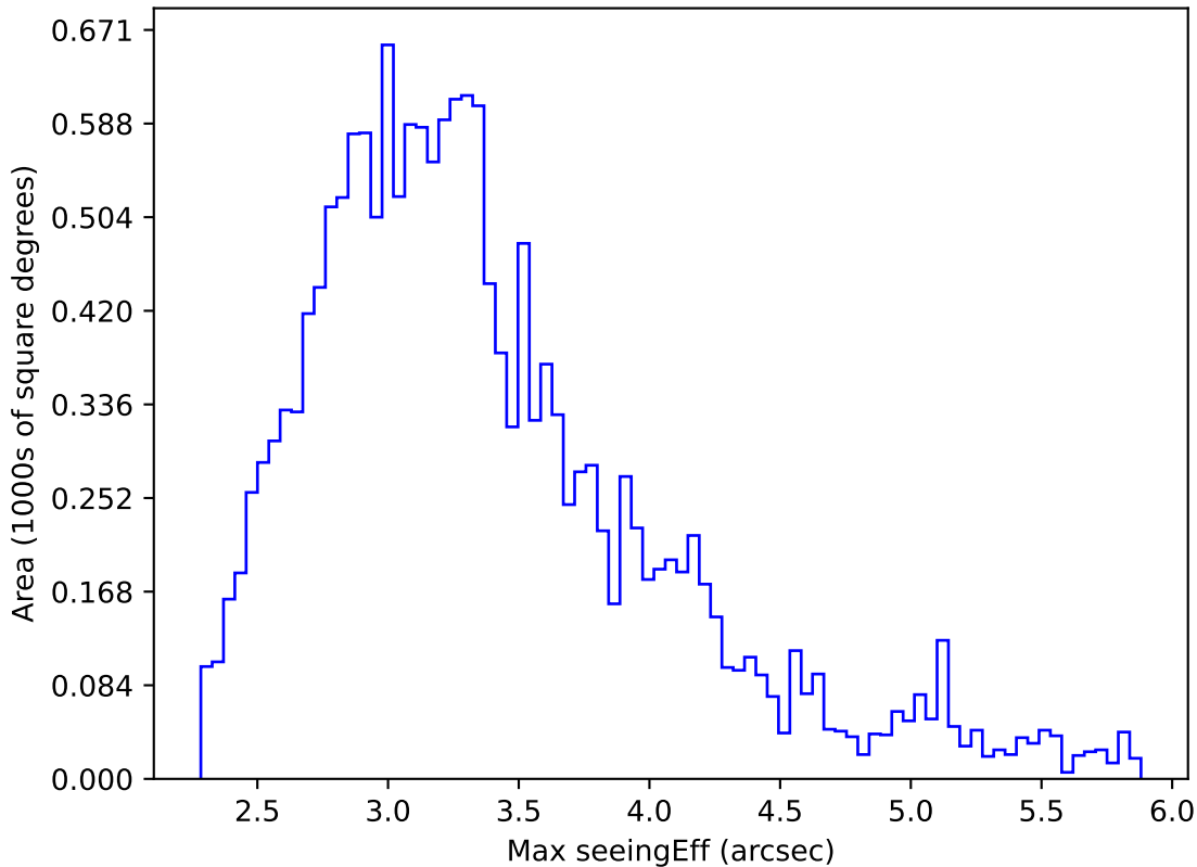
ddf_acor_sf25_lsf30_lsr10_v3.4_10yrs WFD all bands: Max seeingEff
