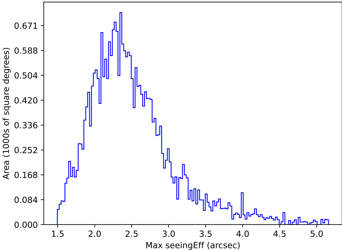
ddf_acor_sf25_lsf30_lsr10_v3.4_10yrs All sky z band: Max seeingEff
