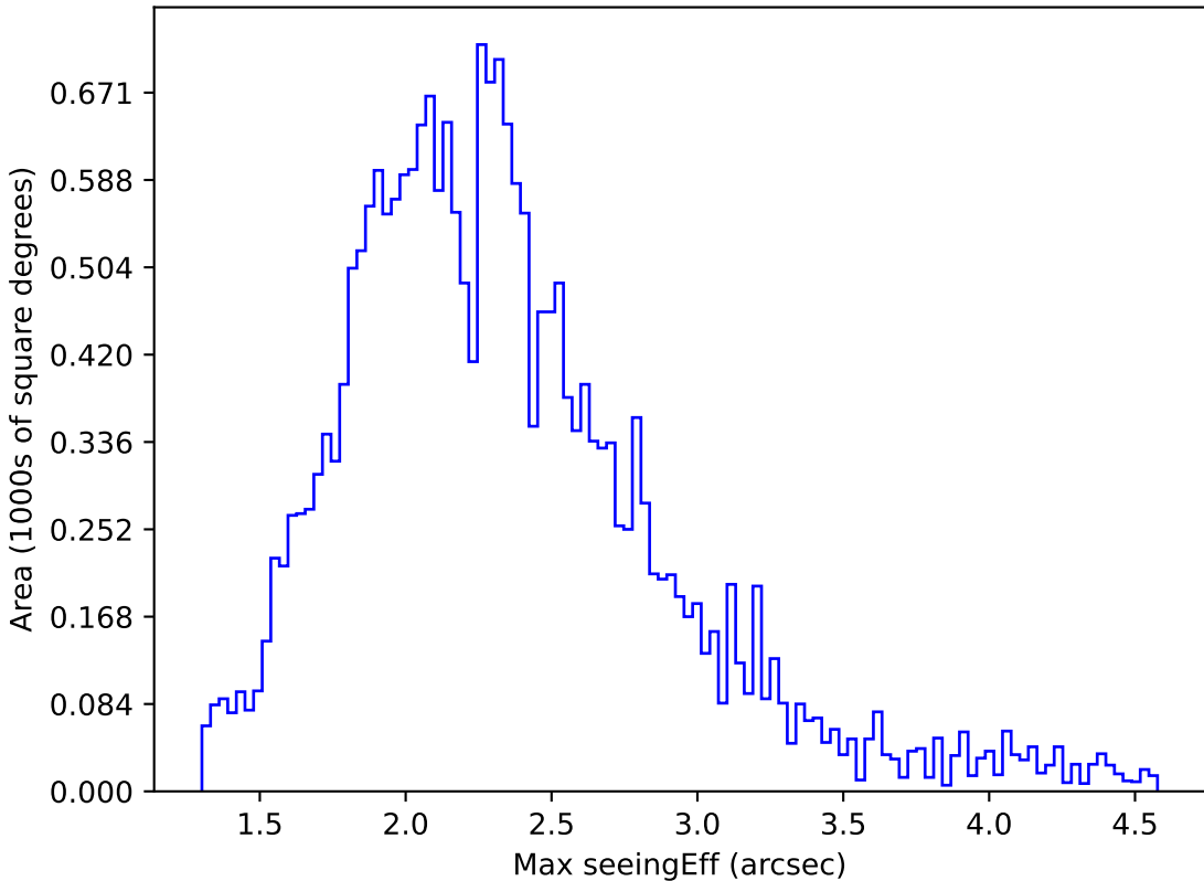
ddf_acor_sf25_lsf30_lsr10_v3.4_10yrs All sky y band: Max seeingEff
