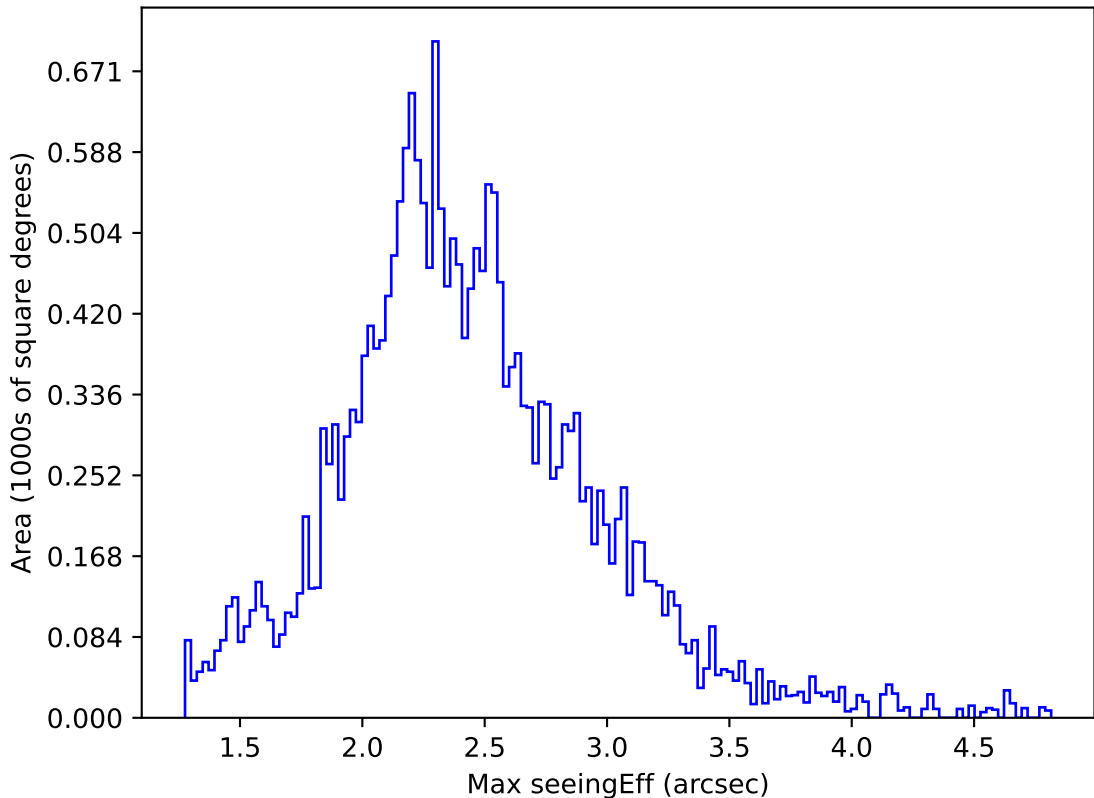
ddf_acor_sf25_ls30_lsr10_v3.4_10yrs All sky u band: Max seeingEff
