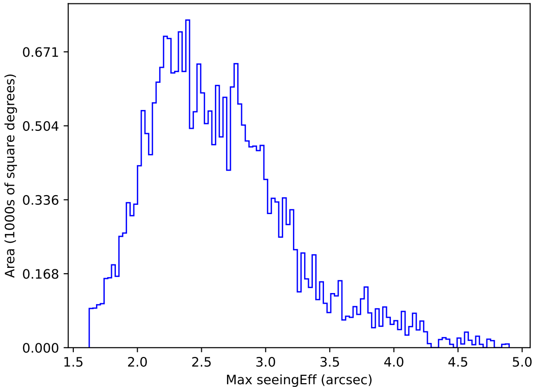
ddf_acor_sf25_lsf30_lsr10_v3.4_10yrs All sky r band: Max seeingEff
