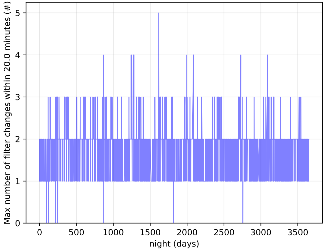
ddf_acor_sf25_Isf30_Isr10_v3.4_10yrs Per Night: Max number of filter changes within 20.0 minutes
