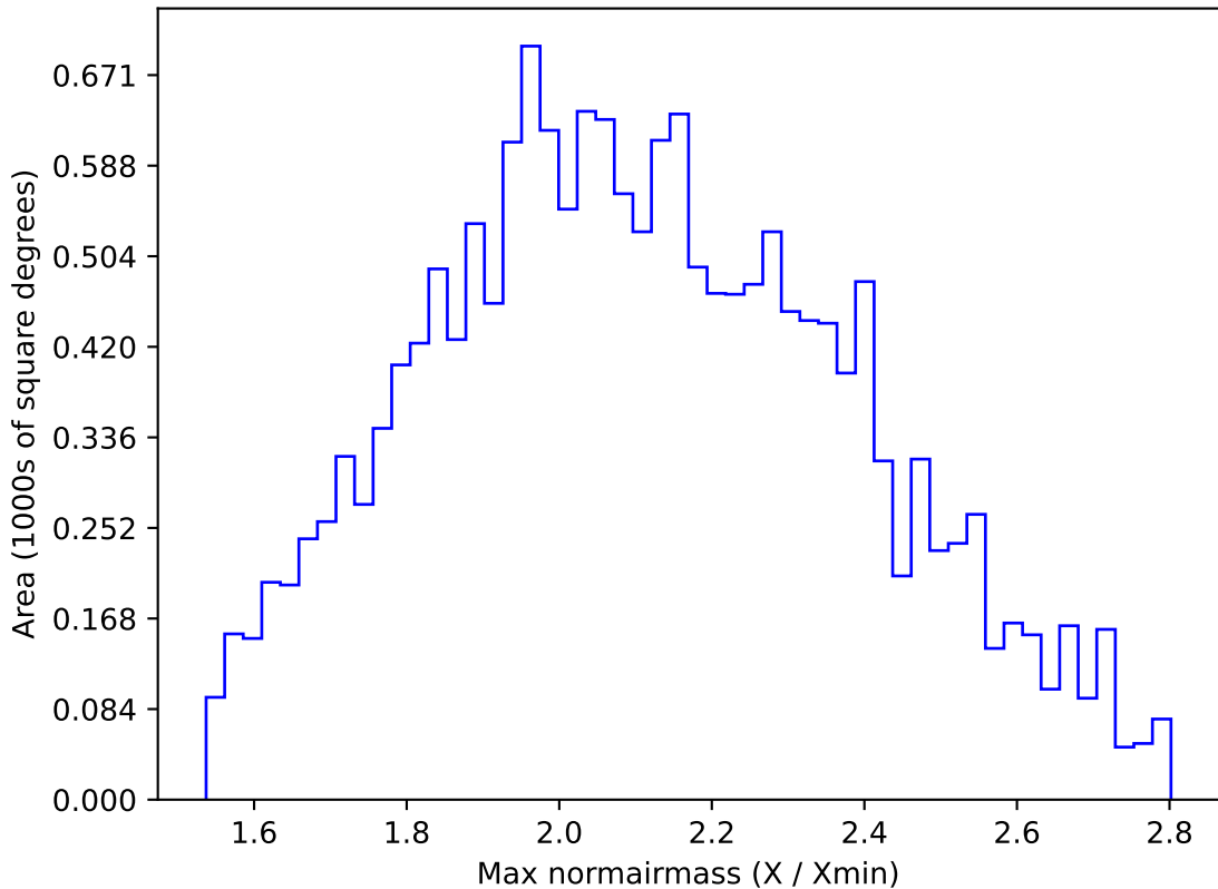
ddf_acor_sf25_lsf30_lsr10_v3.4_10yrs WFD y band: Max normairmass
