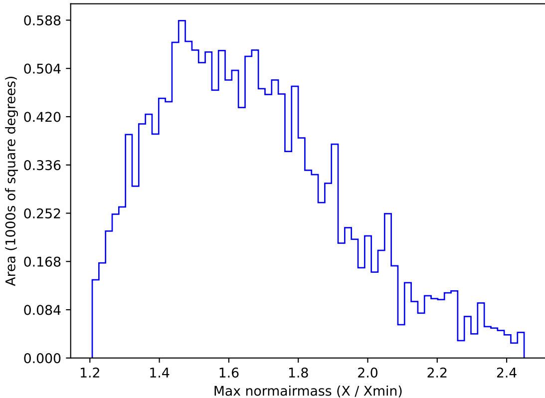
ddf_acor_sf25_lsf30_lsr10_v3.4_10yrs WFD u band: Max normairmass
