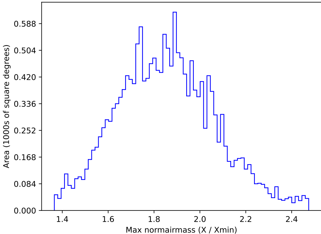
ddf_acor_sf25_lsf30_lsr10_v3.4_10yrs WFD g band: Max normairmass
