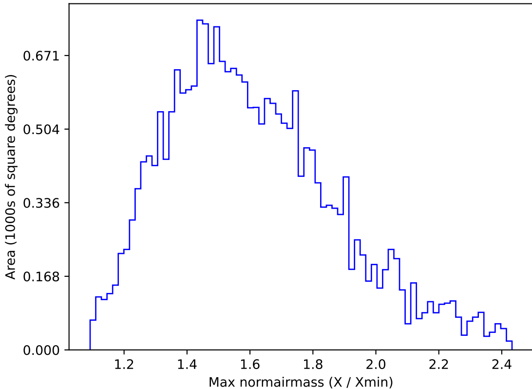
ddf_acor_sf25_lsf30_lsr10_v3.4_10yrs All sky u band: Max normairmass
