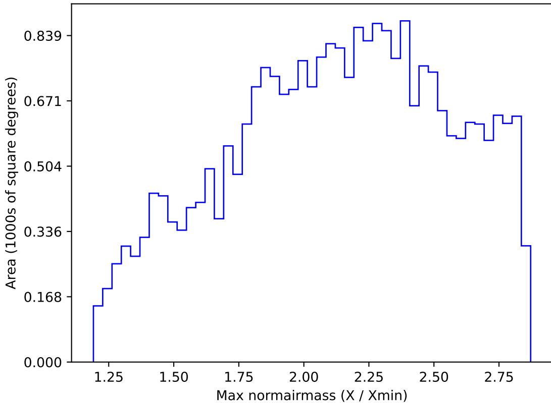
ddf_acor_sf25_lsf30_lsr10_v3.4_10yrs All sky i band: Max normairmass
