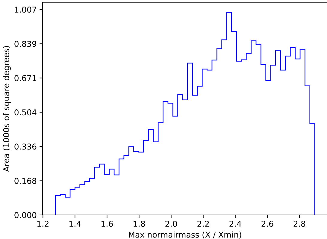
ddf_acor_sf25_lsf30_lsr10_v3.4_10yrs All sky all bands: Max normairmass
