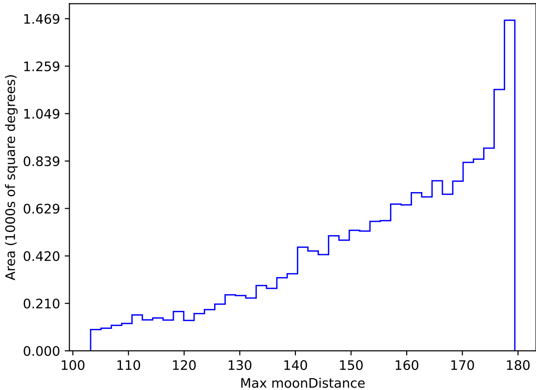
ddf_acor_sf25_lsf30_lsr10_v3.4_10yrs WFD r band: Max moonDistance
