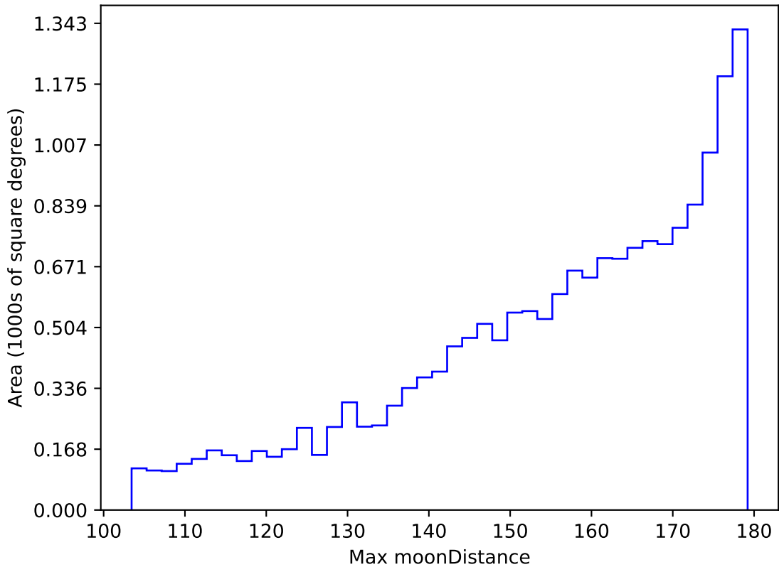
ddf_acor_sf25_lsf30_lsr10_v3.4_10yrs WFD i band: Max moonDistance
