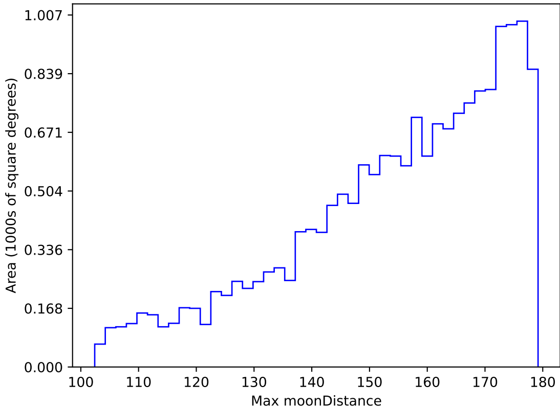
ddf_acor_sf25_ls30_lsr10_v3.4_10yrs WFD g band: Max moonDistance
