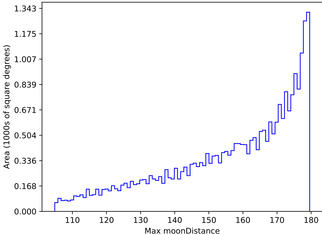
ddf_acor_sf25_lsf30_lsr10_v3.4_10yrs All sky all bands: Max moonDistance
