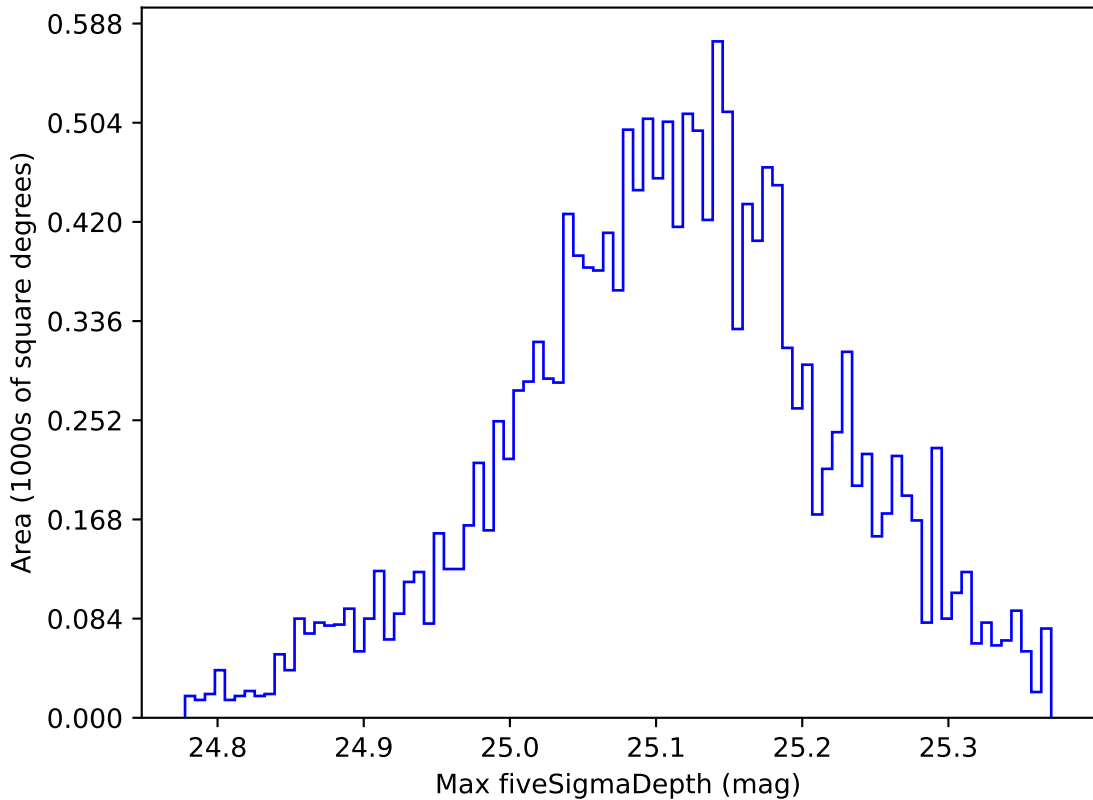
ddf_acor_sf25_lsf30_lsr10_v3.4_10yrs WFD all bands: Max fiveSigmaDepth
