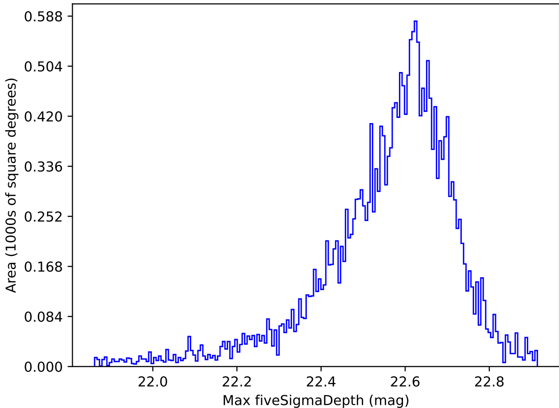
ddf_acor_sf25_ls30_lsr10_v3.4_10yrs All sky y band: Max fiveSigmaDepth
