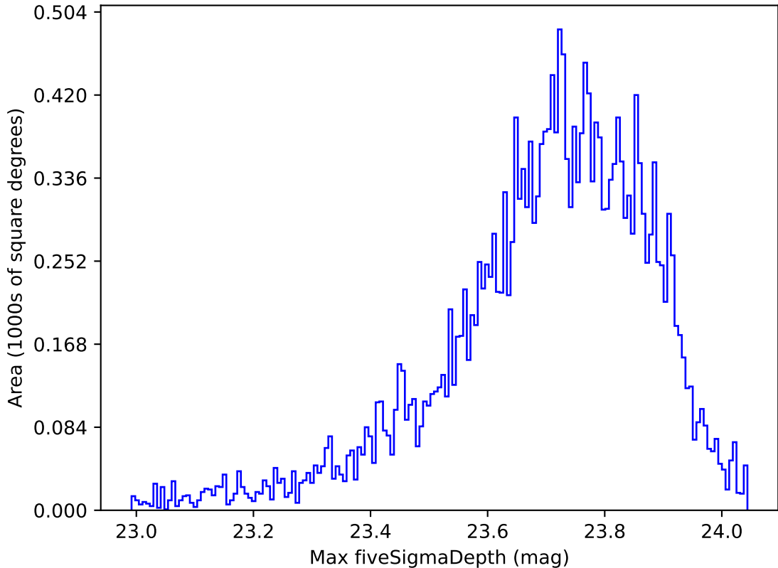
ddf_acor_sf25_lsf30_lsr10_v3.4_10yrs All sky u band: Max fiveSigmaDepth
