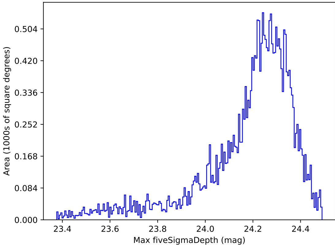
ddf_acor_sf25_lsf30_lsr10_v3.4_10yrs All sky i band: Max fiveSigmaDepth
