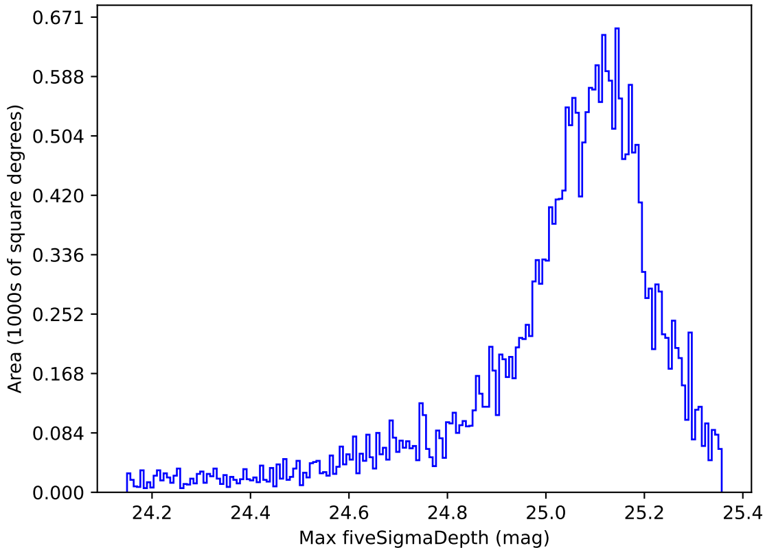
ddf_acor_sf25_lsf30_lsr10_v3.4_10yrs All sky g band: Max fiveSigmaDepth
