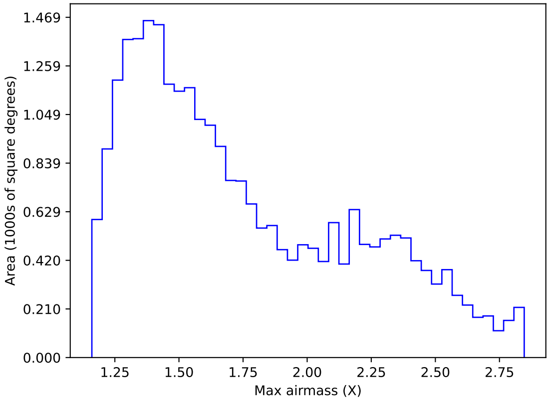
ddf_acor_sf25_lsf30_lsr10_v3.4_10yrs Yr 1 z band: Max airmass
