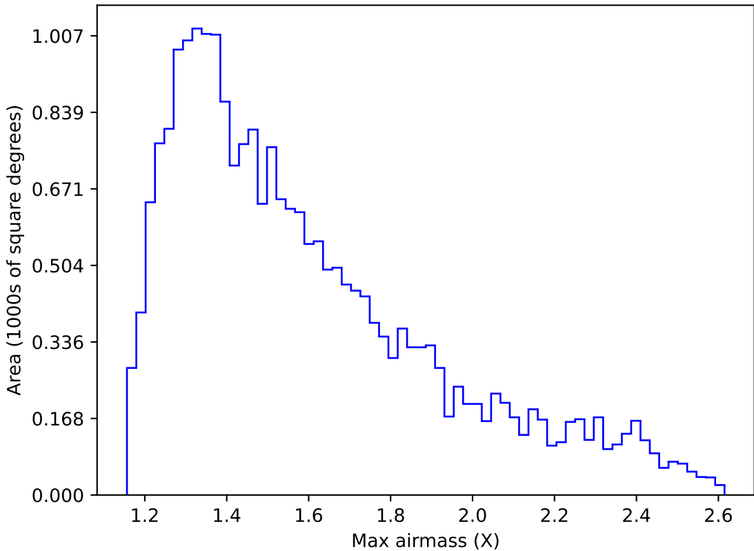
ddf_acor_sf25_lsf30_lsr10_v3.4_10yrs Yr 1 y band: Max airmass
