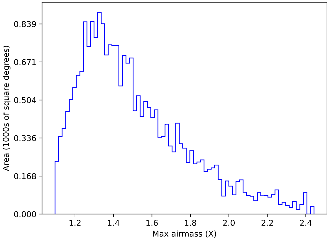
ddf_acor_sf25_lsf30_lsr10_v3.4_10yrs Yr 1 u band: Max airmass
