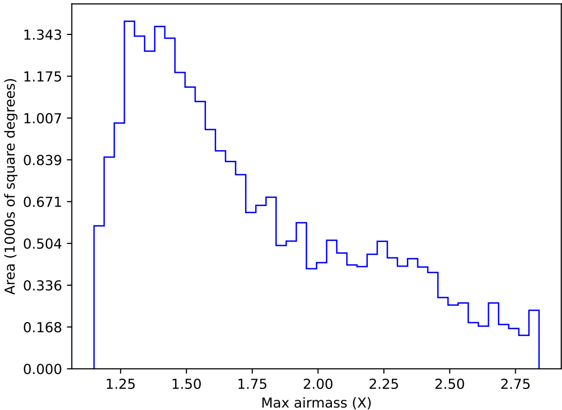
ddf_acor_sf25_lsf30_lsr10_v3.4_10yrs Yr 1 i band: Max airmass
