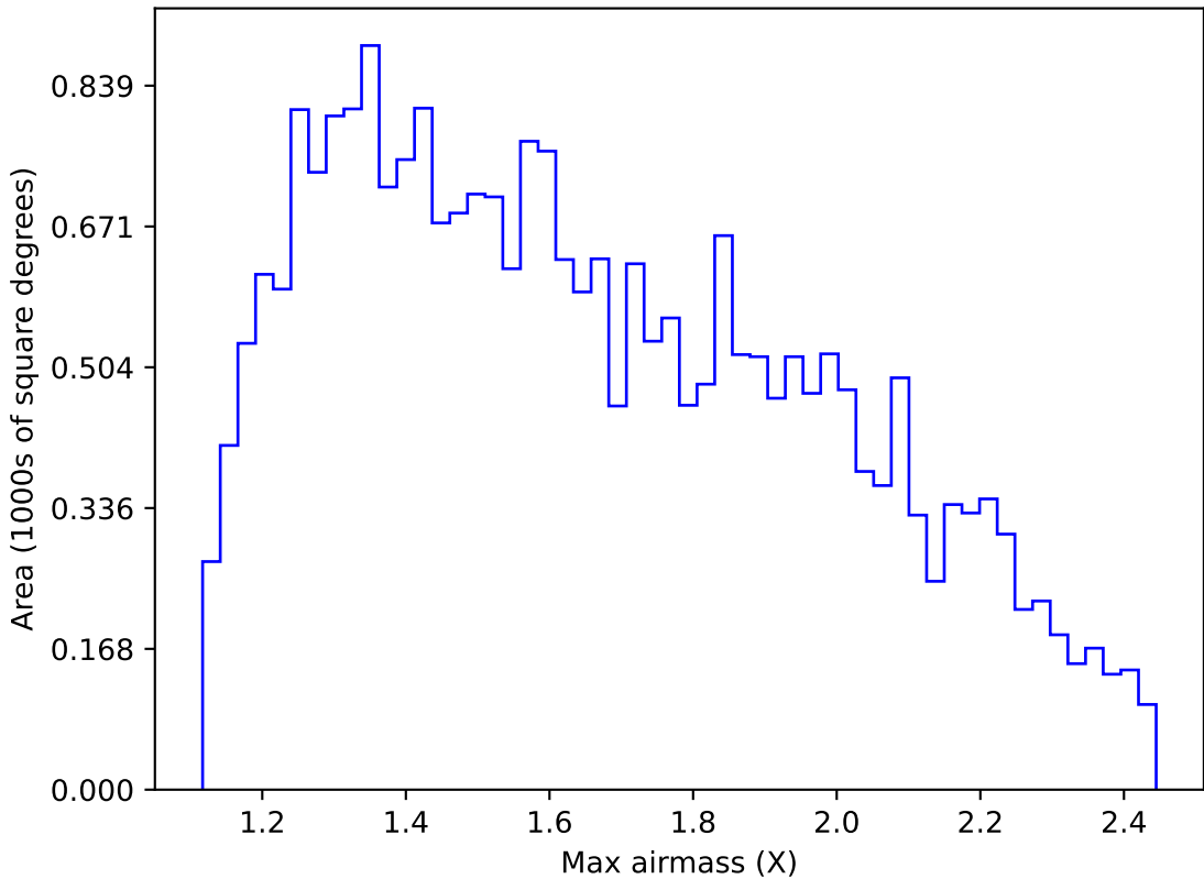
ddf_acor_sf25_lsf30_lsr10_v3.4_10yrs Yr 1 g band: Max airmass
